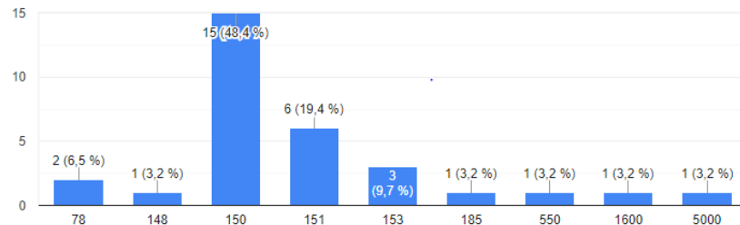
Newsletter
